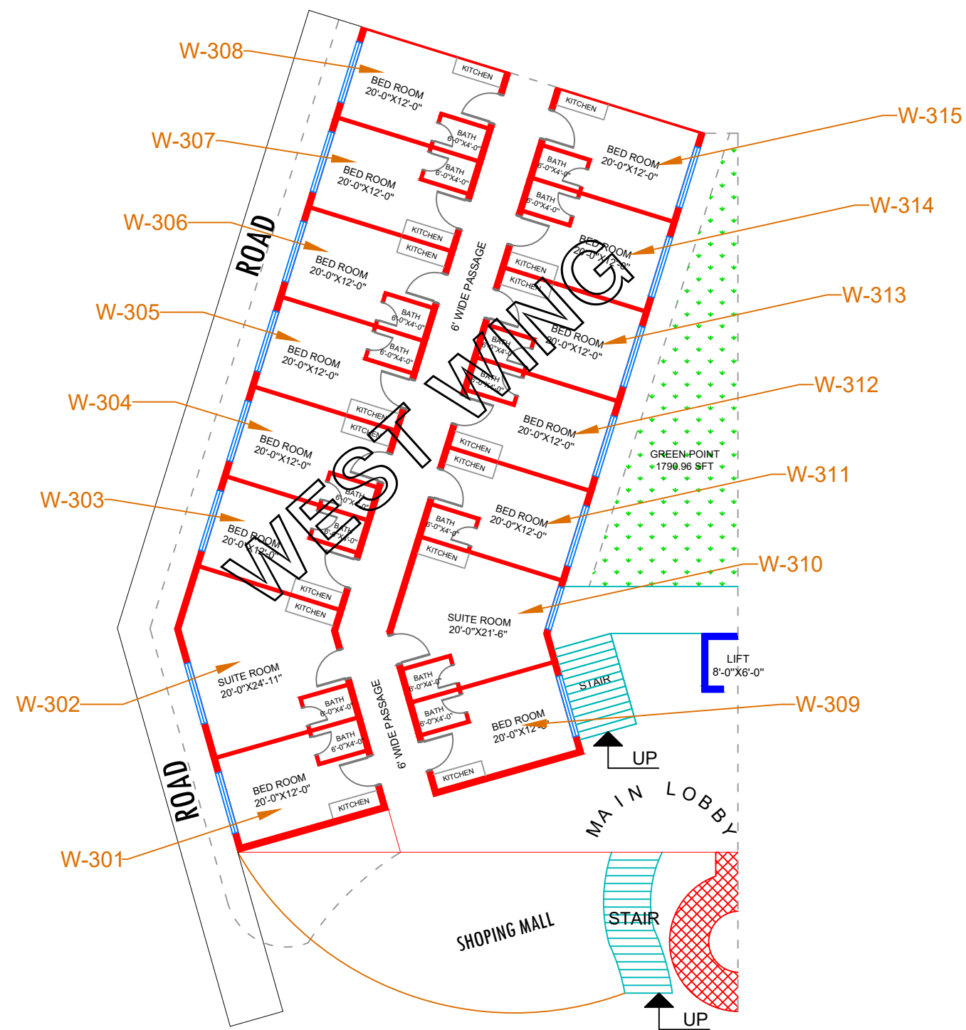
3RD FLOOR PLAN
